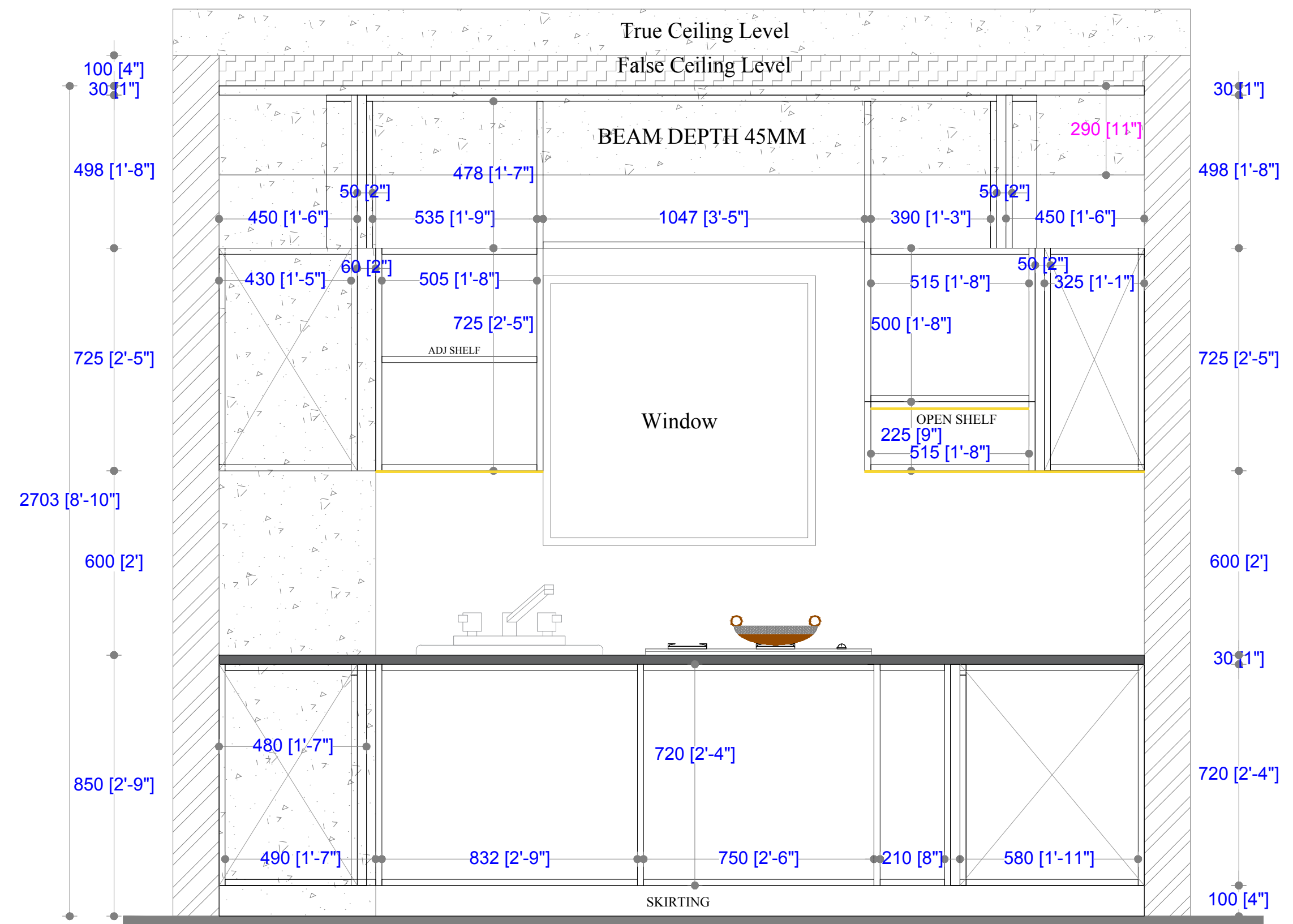
ELEVATION-A (INTERNALS)
