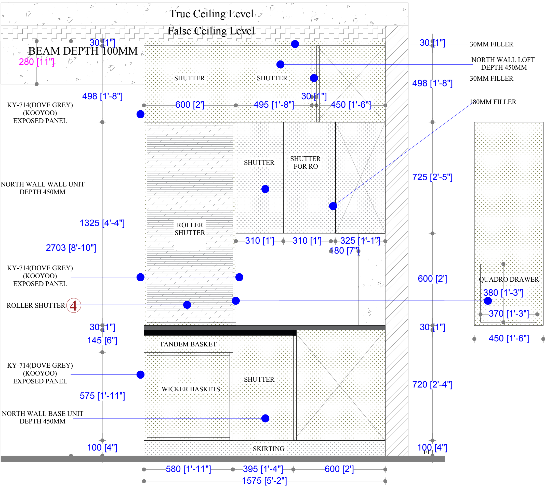
KITCHEN ELEVATION -C (EXTERNALS)
