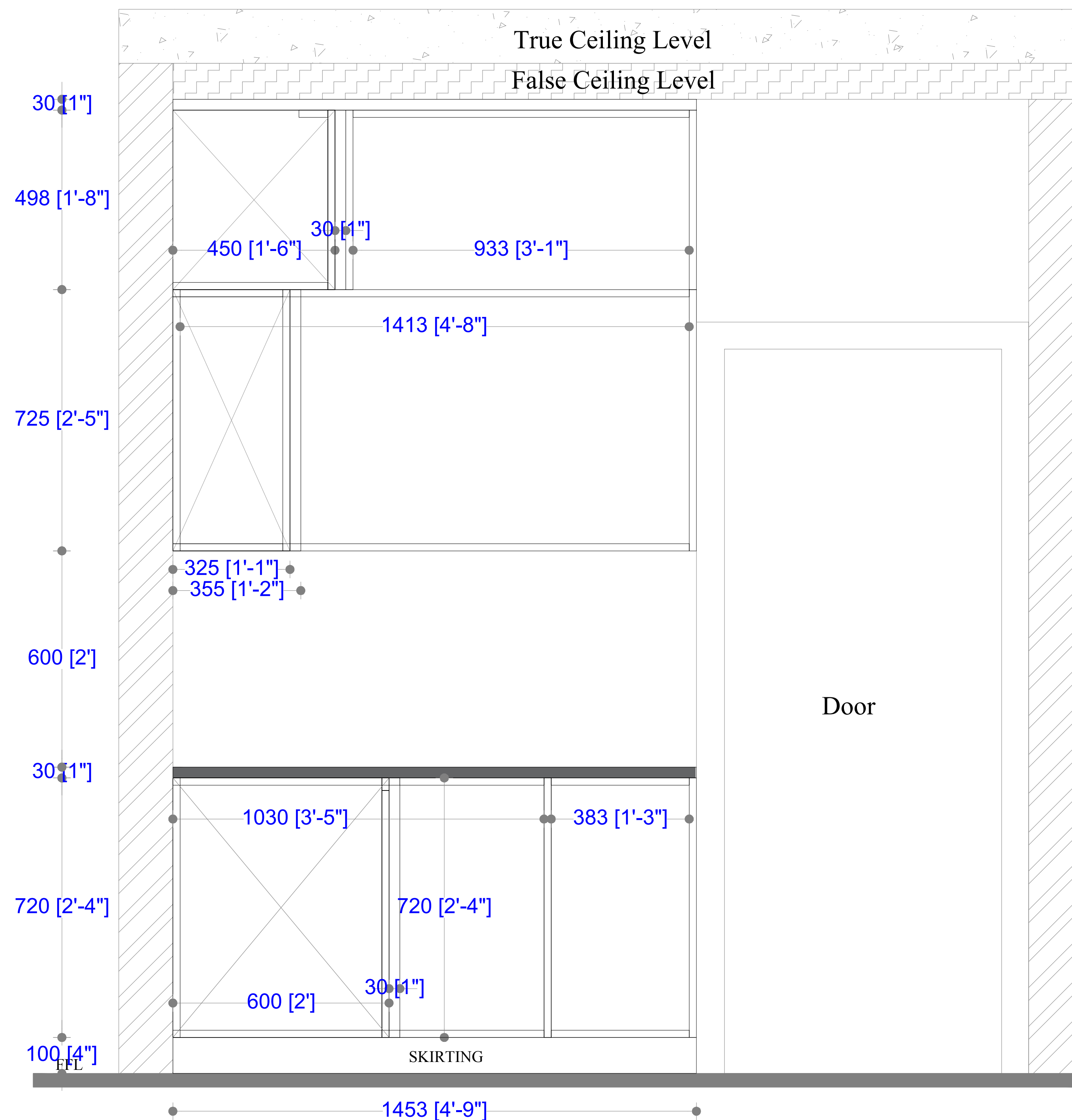
KITCHEN ELEVATION-B (INTERNALS)
