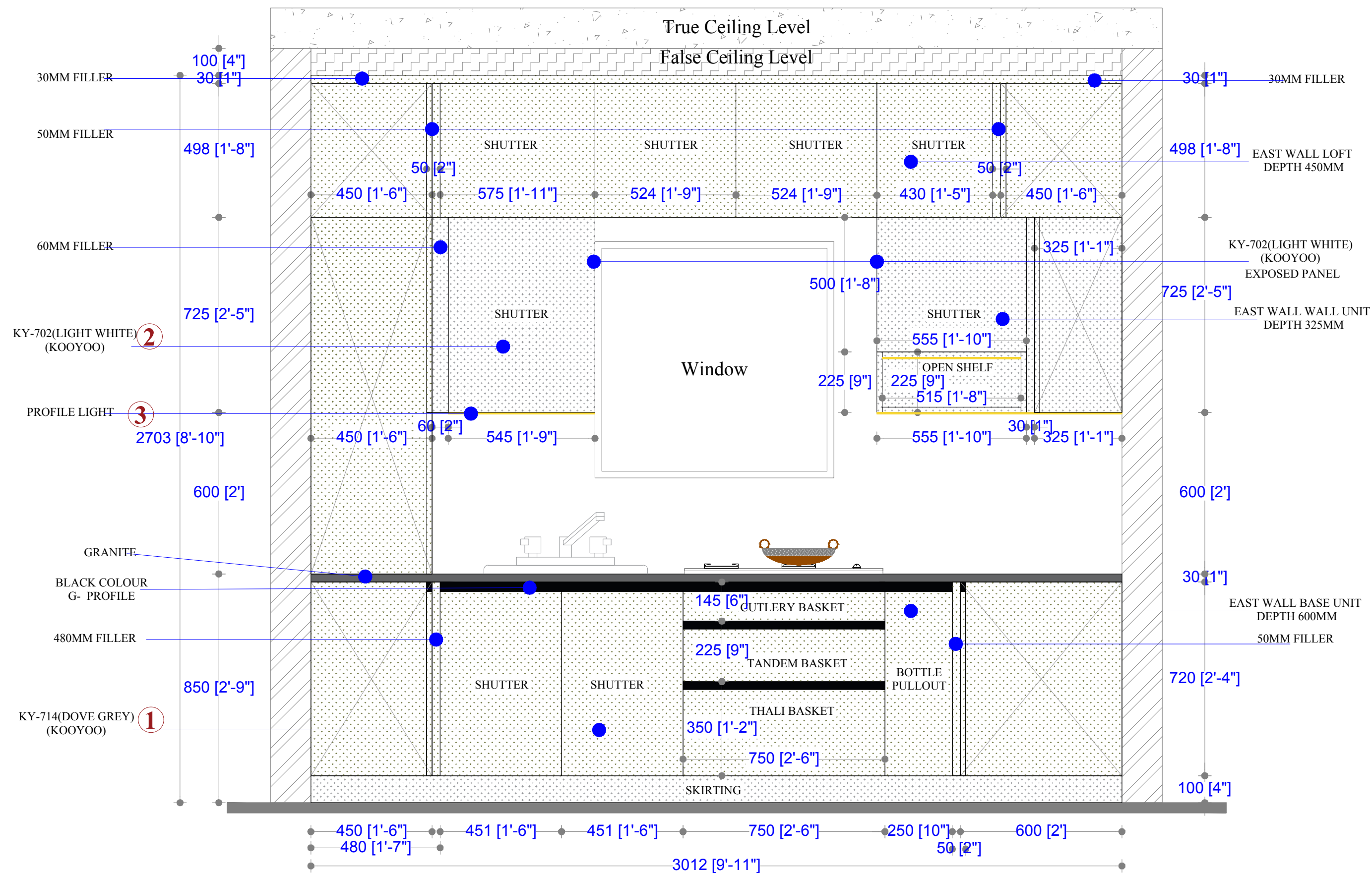
ELEVATION-A (EXTERNALS)
