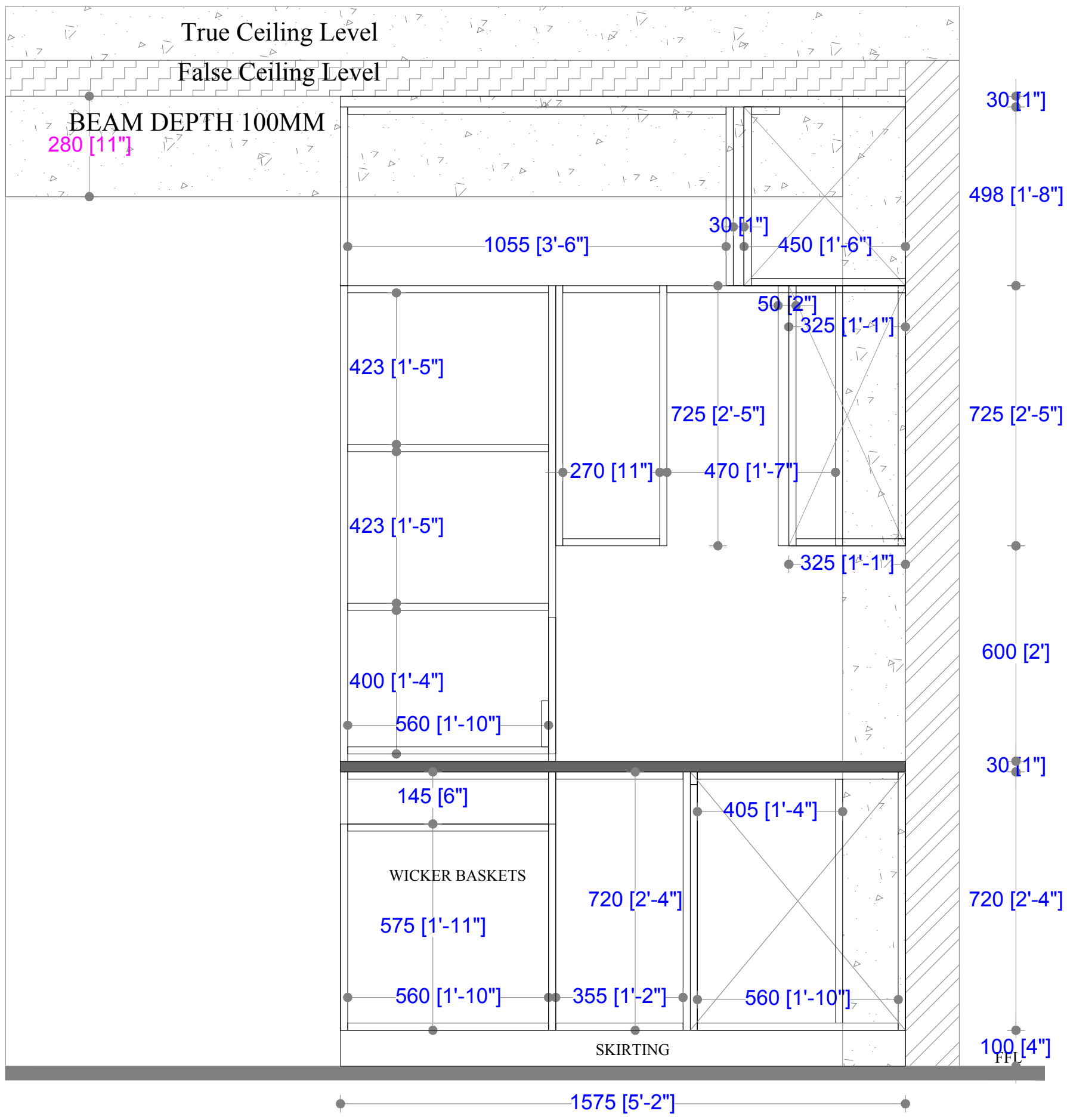
KITCHEN ELEVATION -C (INTERNALS)
