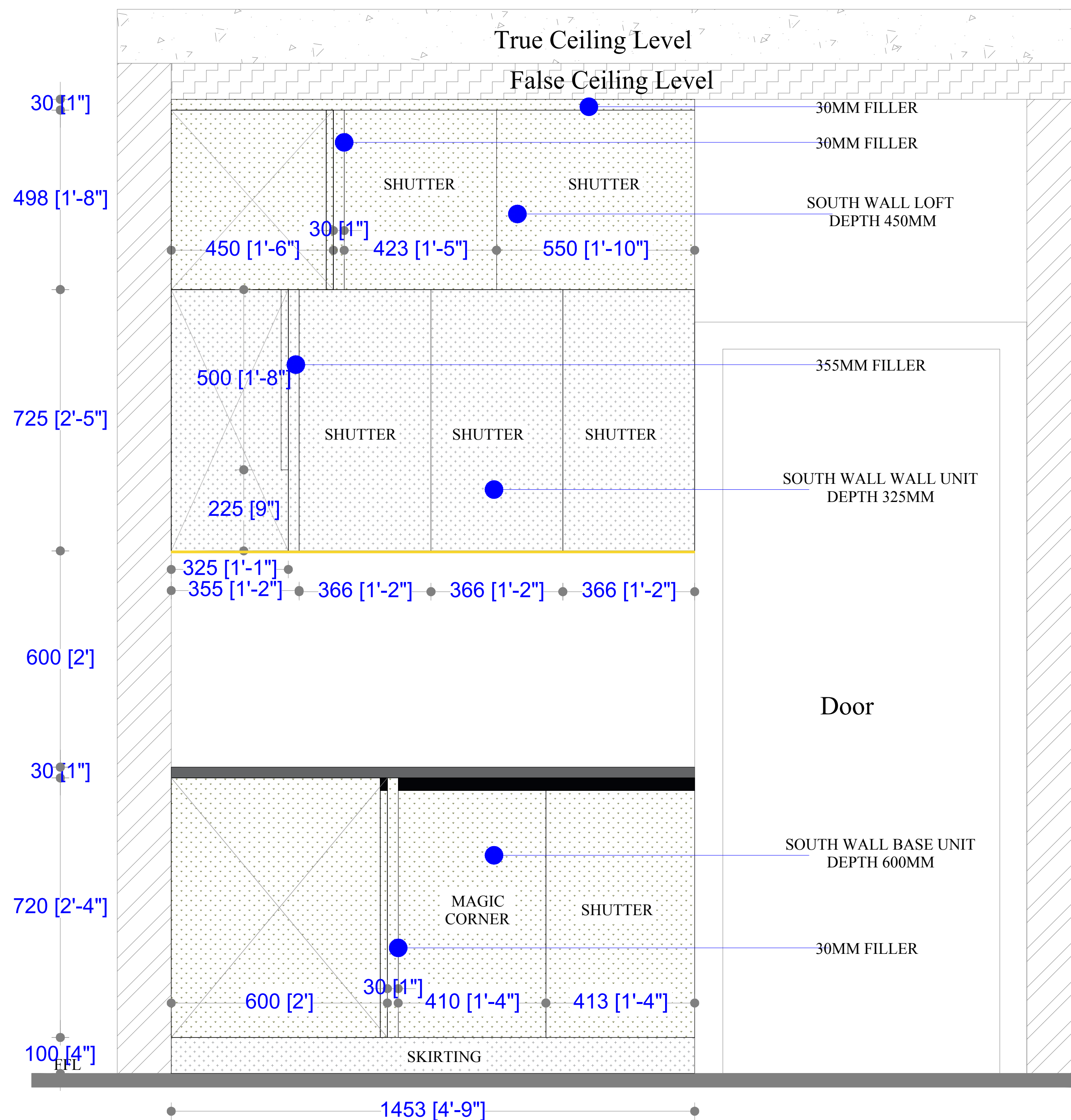
KITCHEN ELEVATION-B (EXTERNALS)
